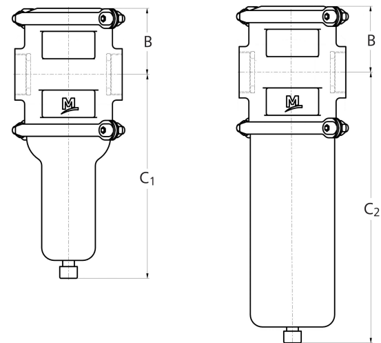
Screwed Connection BSP and NPT
