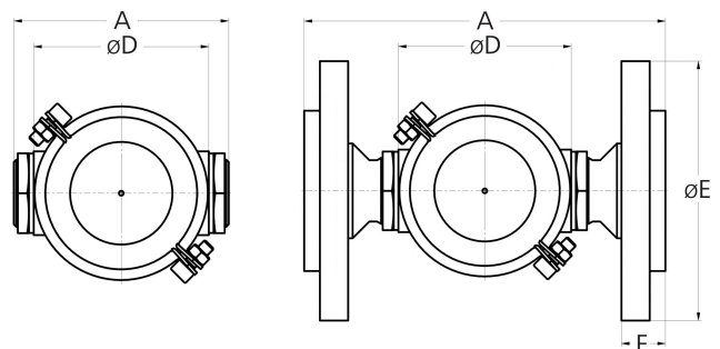
Screwed Connection BSP and NPT
